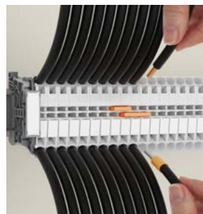
Push-in mode
