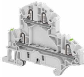
ZK2.5-D2-PE
